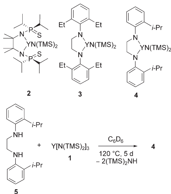
Scheme 2. In situ generation of the yttrium precatalyst for hydroamination.
